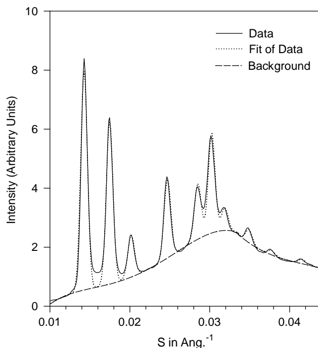
Fig. 2. Plot of scattering intensity for the 2-2 methyl butyl 16:0 PC data. The data is shown as a solid line, the background as a dashed line, and the fit as a dotted line.
