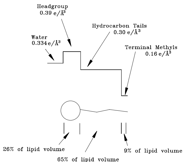
Fig. 5. Electron density model for mono-olein.
