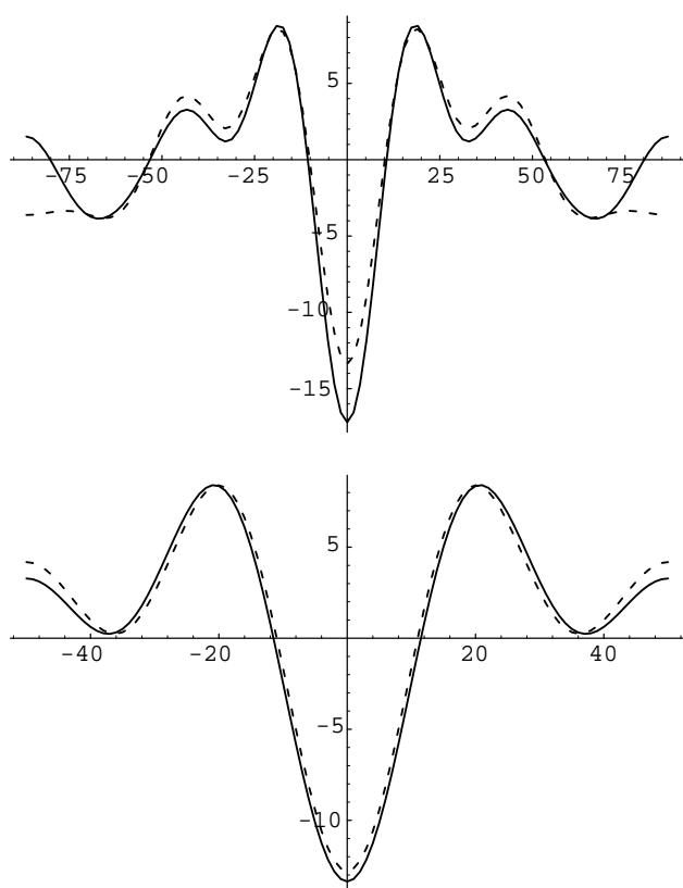
Fig. 12. Data (solid lines) and DOPE model (dashed lines) overlay for 2-2 methyl butyl PC. Top plots: electron density cuts through the flat point. Bottom plots: electron density cuts through the point of maximum curvature.
