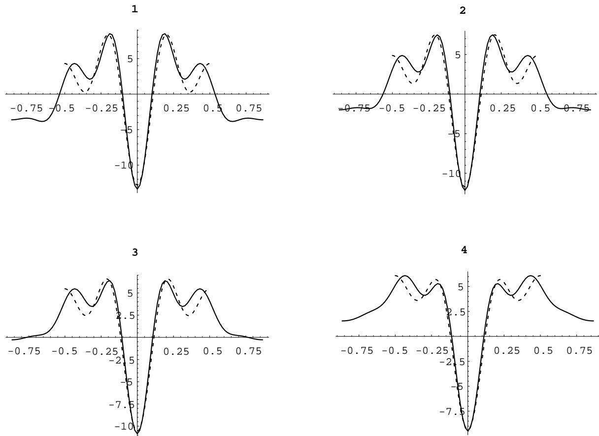
Fig. 8. Plot number 1 contains the electron density cuts for the phospholipid model. Plot number 4 contains the electron density cuts for the same model, except that the headgroup electron density used is from the mono-olein model. Plots 2 and 3 are plots of the electron density cuts for intermediate headgroup electron densities. The x -axes are in Angstroms and the y -axes are in arbitrary units.
