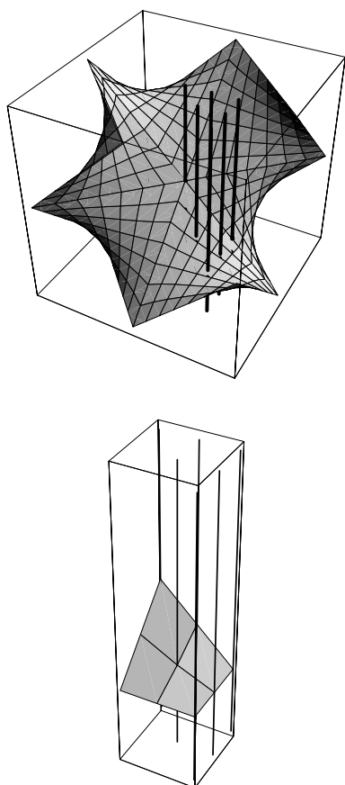
Fig. 3. Top view: unit cell of the D surface. The vertical lines indicate the locations of the electron density minima searches. Bottom view: section of the unit cell pierced by the electron density minima searches.
