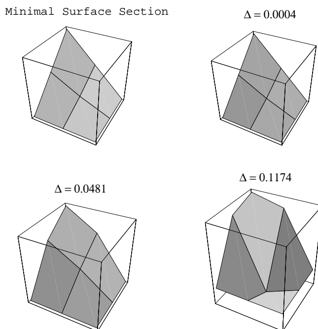
Fig. 4. The top left plot is an actual minimal surface section, with the remaining plots being methyl trough search results for the modeled mono-olein data. The plot on the top right is the methyl trough search result for the correct phasing. \Delta_{\max} is given at the top of each of the methyl trough search plots.
