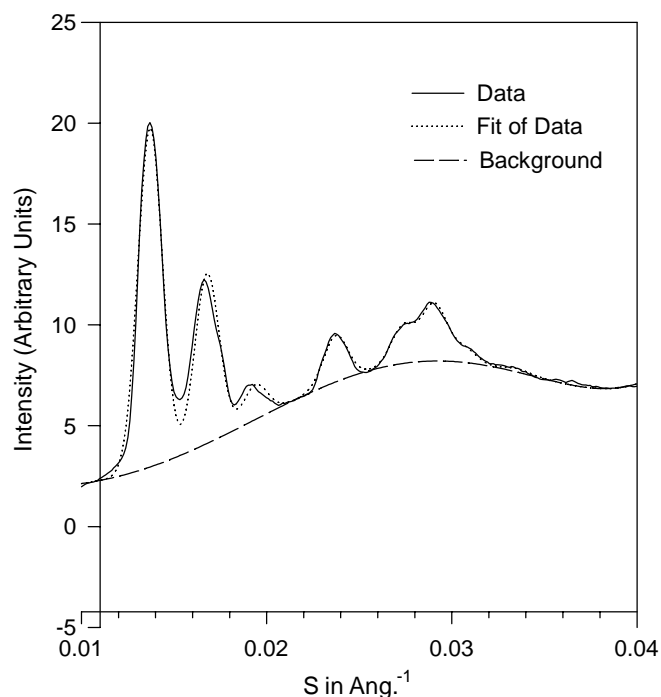
Fig. 1. Plot of scattering intensity for the mono-olein data. The data is shown as a solid line, the background as a dashed line, and the fit as a dotted line.
