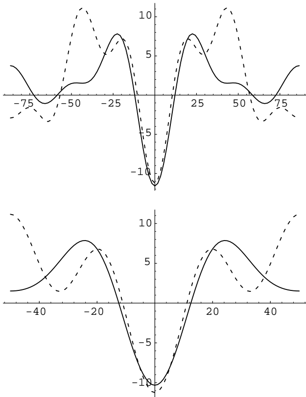
Fig. 10. Data (solid lines) and model (dashed lines) overlay for mono-olein. Top plots: electron density cuts through the flat point. Bottom plots: electron density cuts through the point of maximum curvature.
