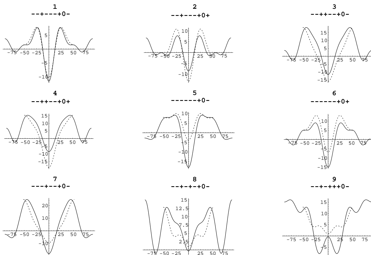
Fig. 9. Electron density cuts for the top nine phasings of mono-olein data from this work. For the phasing at the top of each plot, the solid and dashed lines are perpendicular cuts through the bilayer at the flat point and at a point of maximum curvature, respectively. The x -axes are in Angstroms and the y -axes are in arbitrary units.
