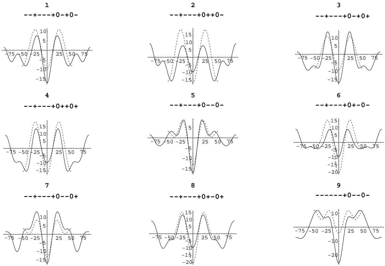
Fig. 11. Electron density cuts for the top nine phasings for 2-2 methyl butyl 16:0 PC. For the phasing at the top of each plot, the solid and dashed lines are perpendicular cuts through the bilayer at the flat point and at a point of maximum curvature. The x -axes are in Angstroms and the y -axes are in arbitrary units.
