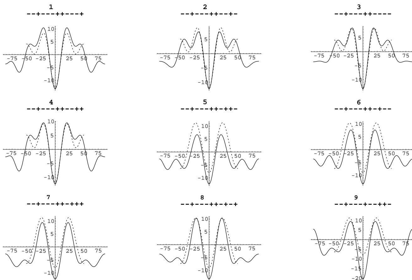
Fig. 7. Electron density cuts for the top nine phasings of modeled phospholipid data. For the phasing at the top of each plot, the solid and dashed lines are perpendicular cuts through the bilayer at the flat point and at a point of maximum curvature. The x -axes are in Angstroms and the y -axes are in arbitrary units.
