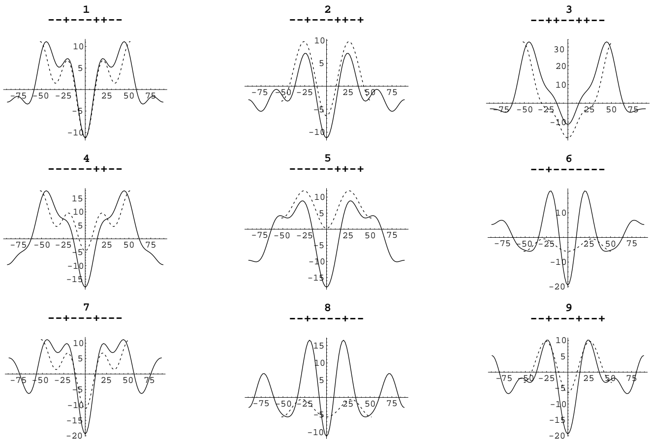
Fig. 6. Electron density cuts for the top nine phasings of modeled mono-olein data. For the phasing at the top of each plot, the solid and dashed lines are perpendicular cuts through the bilayer at the flat point and at a point of maximum curvature. The x -axes are in Angstroms and the y -axes are in arbitrary units.
