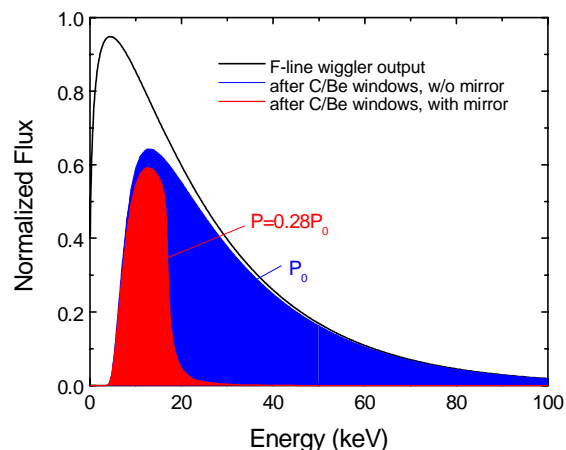
Figure 2. Calculated comparison of F-line wiggler outputs with and without the installation of the white-beam collimating mirror, showing a reduction of power P_0 by more than a factor of three.
