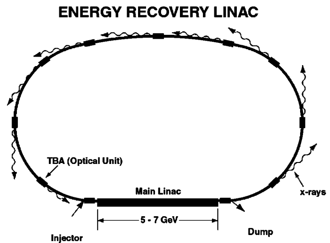
FIG. 1. Schematic layout of an ERL. The electrons are injected into a superconducting linac and then routed by electron optics (e.g., TBA=triple bend achromats, etc.) through undulators to produce SR. The bunches then decelerate in the linac and are bent aside by a weak dipole into a beam dump. Bunch compressors and decompressors (not shown) in the loop are used to produce very short bunches.
