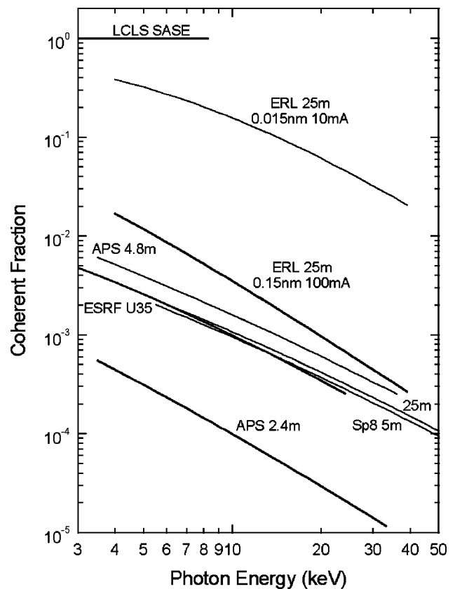
FIG. 3. Comparison of calculated coherent fractions of the various sources with photon energy.
