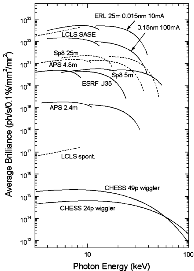
FIG. 2. Comparison of calculated average spectral brilliance of the various sources. The parameters used for undulator sources are listed in Table I. The CHES wiggler sources assume 5.3 GeV 300 mA operation and a FWHM source size of d_x=5.5 mm and d_y=0.9 mm for the 24-pole wiggler at the F line and d_x=3.3 mm and d_y=0.85 mm for the 49-pole wiggler at the A/G line.
