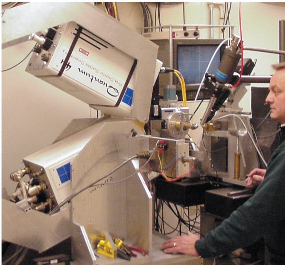
Figure 5: Installation of a dual Quantum-4 detector system at F1 station by Bill Miller and other MacCHESS staff members. The two detector assembly, designed by Mike Cook, is capable of independent rotation by up to 30 degrees, effectively producing a detector with a total (V-shaped) surface area of 380 x 190 mm.
