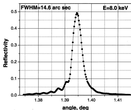
Figure 6: Reflectivity curve from the Osmic low-contrast multilayer with 500 bi-layers and d = 31.5 \text{ \AA} . The width of the curve is 14.6 arc sec, bandwidth \Delta E/E = 0.29\% . Data taken at CHESS A2 station.
