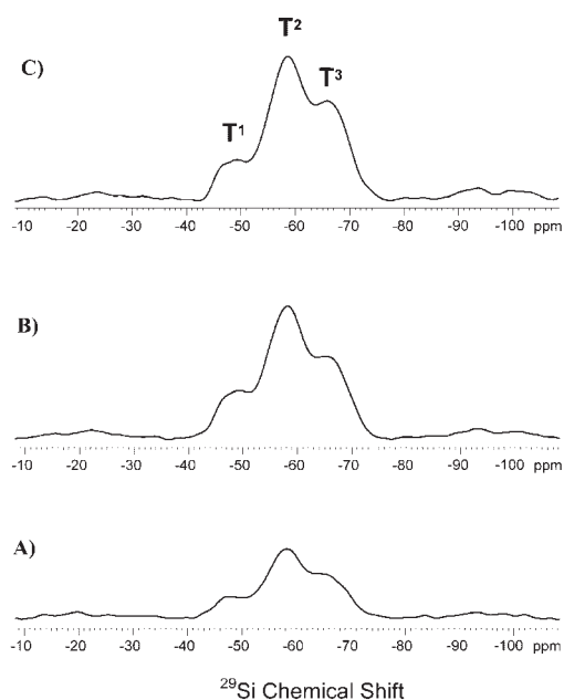
Figure 7. ^1\text{H} - ^{29}\text{Si} CP-MAS spectra of different hybrid materials with A) spherical morphology B) cylindrical morphology and C) lamellar morphology. Reference: \text{Si}[\underline{\text{Si}}(\text{CH}_3)_3]_4 = -9.8 ppm.
