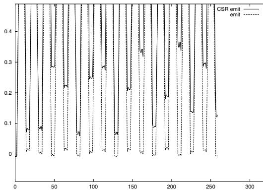
Figure 4: CSR emittance growth in the return loop. Solid: with CSR, dashed: without radiation. Units are % of 0.1nm along the linac (in m).
