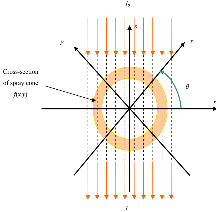
Fig. EPAPS1b. Parallel x-ray beam penetrating spray cone and coordinate systems.
