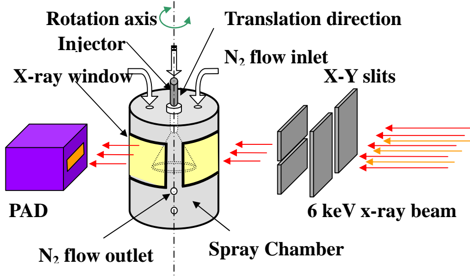
Fig. EPAPS1a. Schematic of experiment setup.
