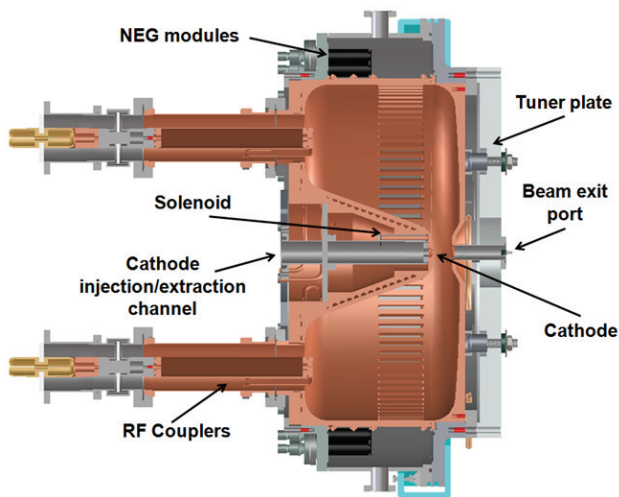
Figure 7: Low frequency, normal-conducting CW gun developed at LBNL [12, 13].
