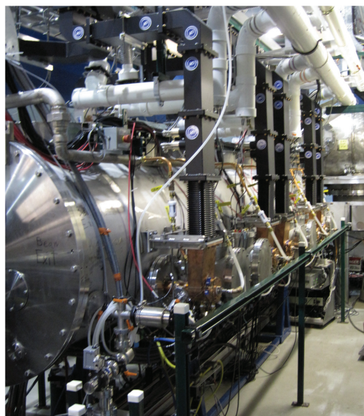
Figure 4: Superconducting booster module of the Cornell ERL injector, capable of providing beam powers of up to 500 kW via five two-cell cavities.
