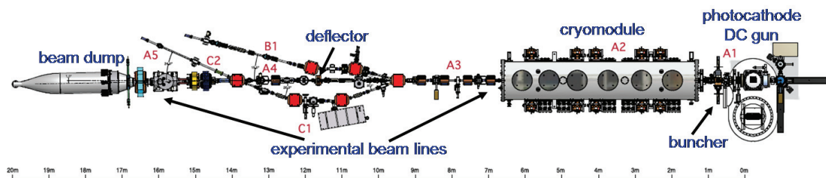
Figure 2: Schematic of the Cornell high current injector consisting of a DC gun, a buncher cavity, a cryomodule containing five 2-cell superconducting 1.3 GHz cavities, subsequent beam lines for a beam characterization followed by a high power beam dump.
