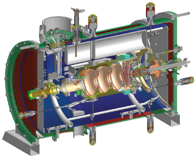
Figure 8: Schematic of the superconducting ELBE photoinjector (from [15]).
