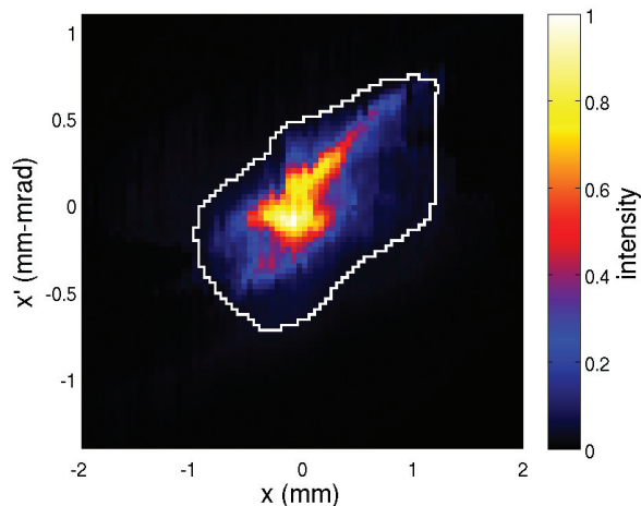
Figure 6: Horizontal phase space distribution measured at the high current Cornell ERL test injector for q = -77 pC, E_{\text{kin}} = 9.7 MeV during the first commissioning. The normalized rms emittance is \varepsilon_x = 2.7 mm mrad, dominated by a beam halo. For the beam core containing 90 % of the particles (indicated by the white line), we receive \varepsilon_{x,90} = 1.6 mm mrad.
