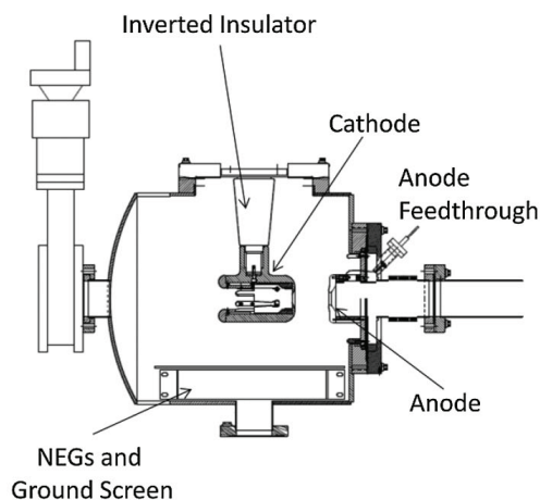
Figure 3: Schematic of an “inverted” DC gun (from [6]).
