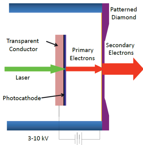
Figure 10: Principle of the diamond amplifier (from [18]).
