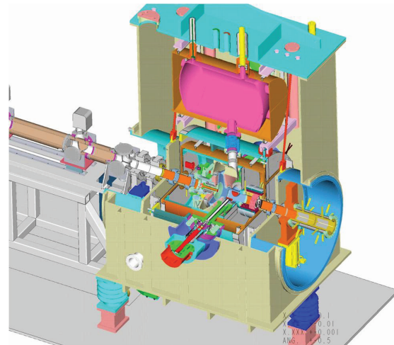
Figure 9: High-current superconducting gun developed at BNL (from [16]).
