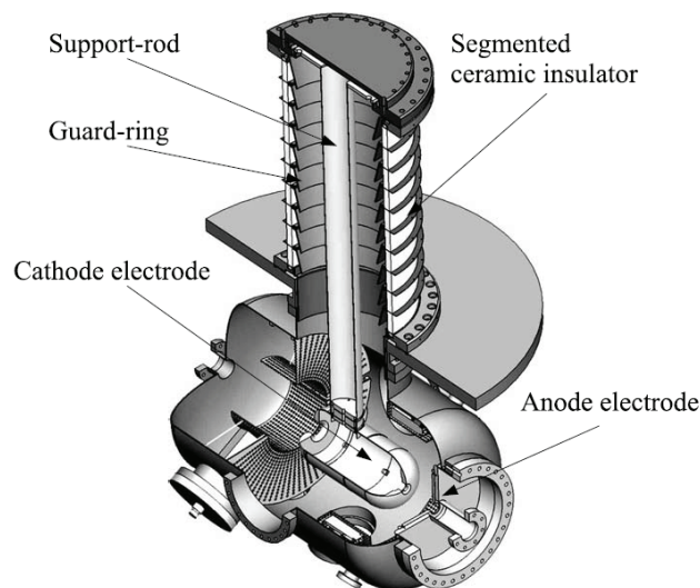
Figure 1: Design of a DC gun in which a segmented insulation ceramics with guard-rings is applied to prevent field emission bursts damaging the ceramics (from [4]).
