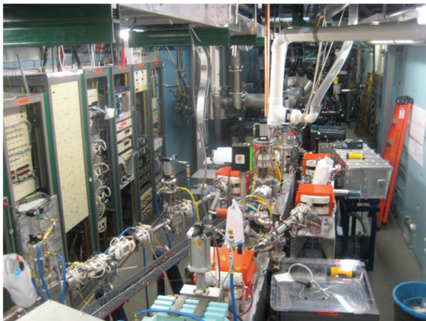
Figure 5: Diagnostics section of the Cornell ERL injector, including emittance measurement systems, a transverse deflecting cavity to study the longitudinal phase space, several view-screens, high current wire-scanners (not yet commissioned), as well as BPMs and beam loss monitors.
