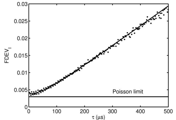
Figure 10 Fractional RMS fluctuation of the CHESS G3 beam intensity versus correlation time. The solid line is a fit to \text{FDEV}_I^2 = A\tau^2 + P .
